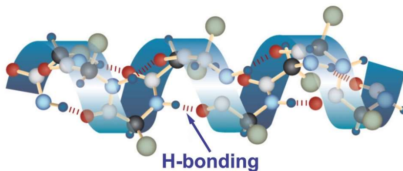
Figure 10: The H-bond breakdown allows enthalpy work to proteins by H-bond breakdown, allowing transitional changes to a protein like (adenylate cyclase) AC. A proline allows bending and sliding with H-bonds breakdown play the role of activation energy with release of dimers. At each transitional state of AC the new configurations respond to a sequence of coordinative state first with Mg^{2+} to create AMP and them replacing Mg^{2+} by Ca^{2+} and a new configuration of coordinative R-groups, allowing cycling to cAMP to AMP and release of water dimers.
