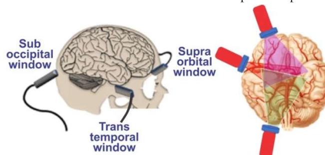
Figure 12: illustrates the available acoustic windows for insonation and the spread of ultrasound waves across Circle of Willis through the available acoustic windows. Abbreviations: V_{max} , maximal cerebral blood flow velocity; V_{min} , minimal cerebral blood flow velocity; MBFv , mean blood flow velocity; MBFv(b) , mean blood flow velocity at baseline; MBFv(r) , mean blood flow velocity during/after hypercapnic stimulus; VMR , vasomotor reactivity; CVC , cerebrovascular conductance index; CVR , cerebrovascular resistance index; SBP , systolic blood pressure; DBP , diastolic blood pressure; MAP , mean arterial pressure; PI , pulsatility index; PR , pulsatility ratio; CPP , cerebral pulse pressure [48].
