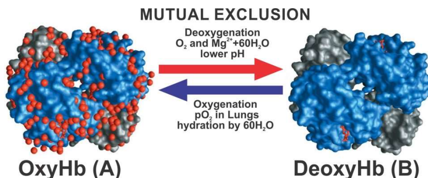
Figure 4: Mutual exclusion prevents the two forms of Hb to coexist at the same time for that the loss of 60 molecules of water is a vectorial transition from oxyHb to deoxyHb in the circulatory system that adds an energy barrier the location requirement. R-residues of Hb participate to form by mutual exclusion a two chelating sites for 2Mg^{2+} in oxyHb. Transition from oxyHb associated to 60 molecules of waters (A) to a dehydrated loss of water molecules in deoxyHb (B) associated to binding site in deoxyHb for 2,3-DPG, increasing and decreasing affinity for O_2 , respectively [18].
